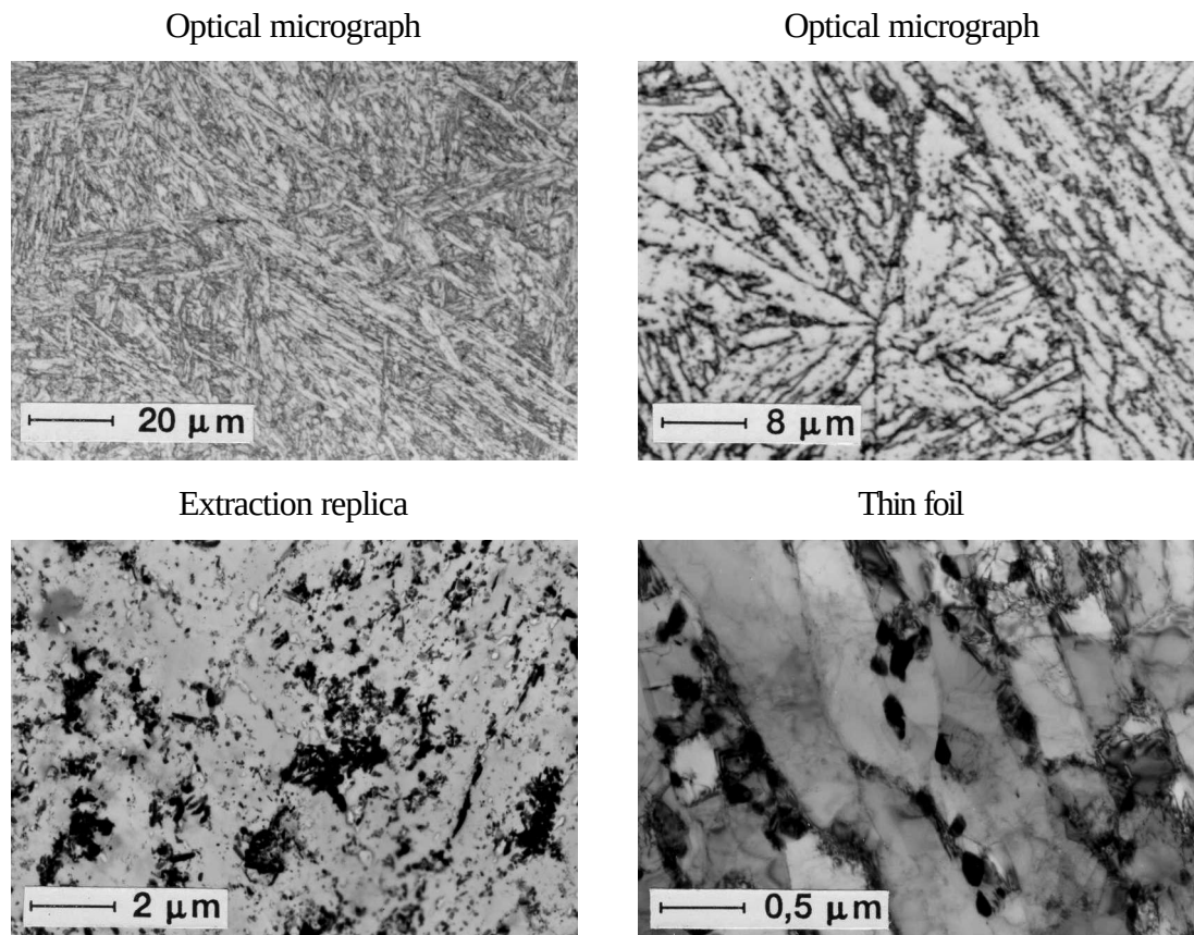
Figure 9: Microstructure of X11CrMoWVNb9-1-1 (T/P911).
